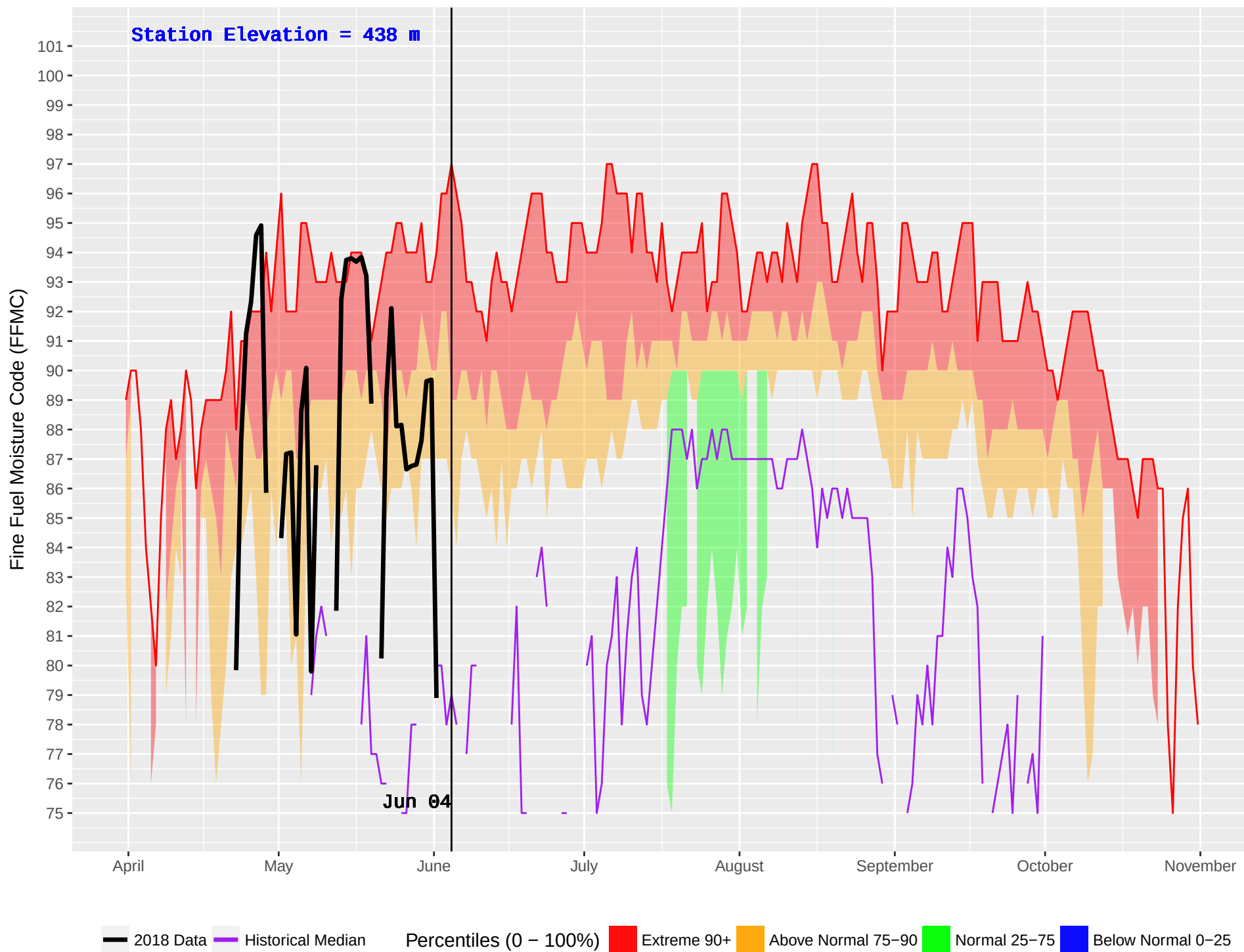
MENZIES CAMP (19) : Historical (1970–2016) and Current (2018) Noon Fine Fuel Moisture Code (FFMC)
