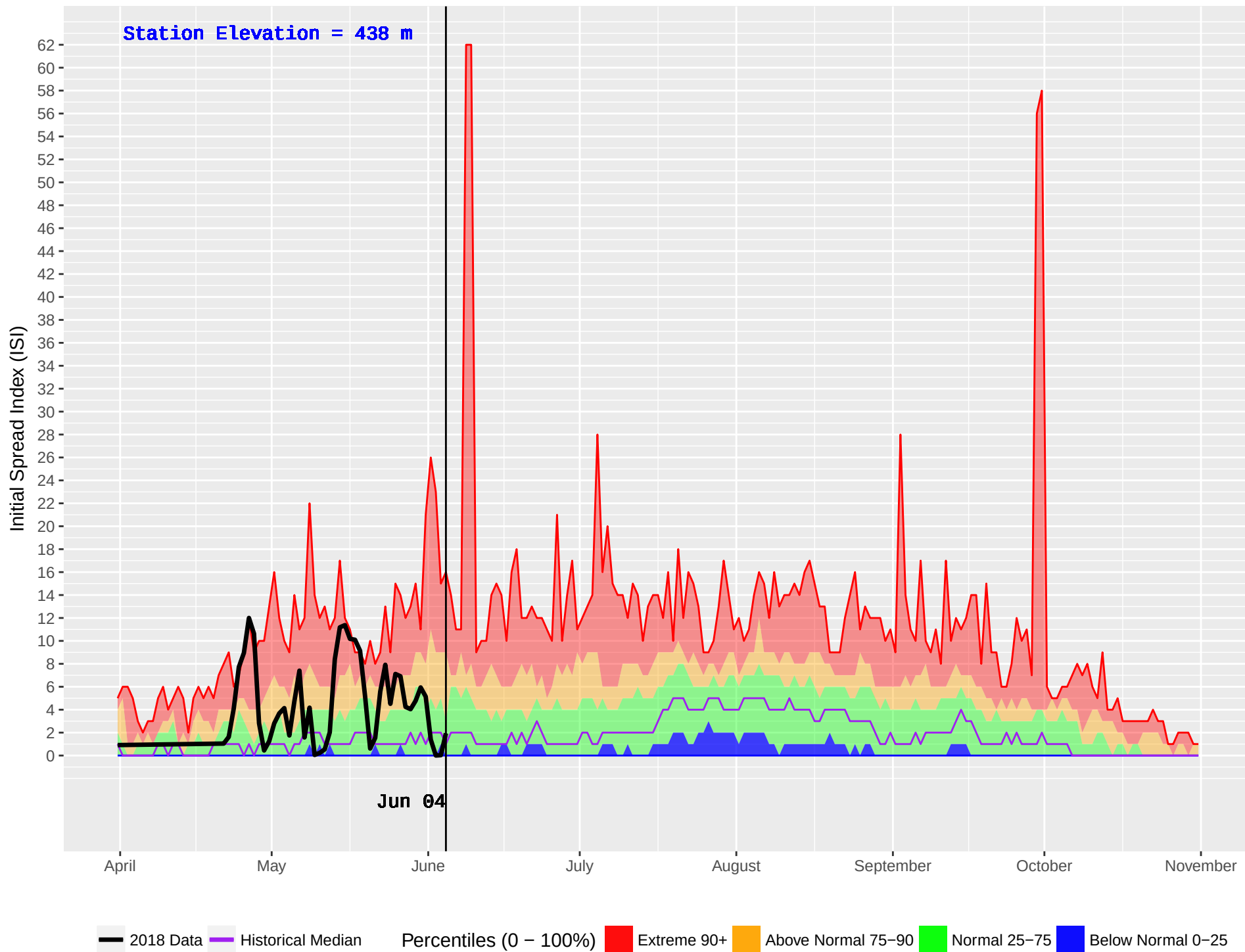
MENZIES CAMP (19) : Historical (1970–2016) and Current (2018) Noon Initial Spread Index (ISI)
